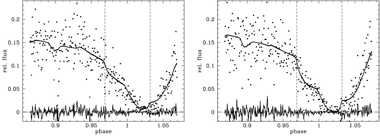
Fig. 10. Extracted CIV light curves and best fits. Left: orbit 1, right: orbit 2. In each panel, ten light curves from different fit runs are overplotted (hard to recognize) to show the stability of the fit. The residuals are scaled down by a factor of 4 for clarity. The vertical dashed lines mark the ingress and egress of the white dwarf and, hence, approximately the begin of the ingress and egress of the magnetically funneled accretion stream.
